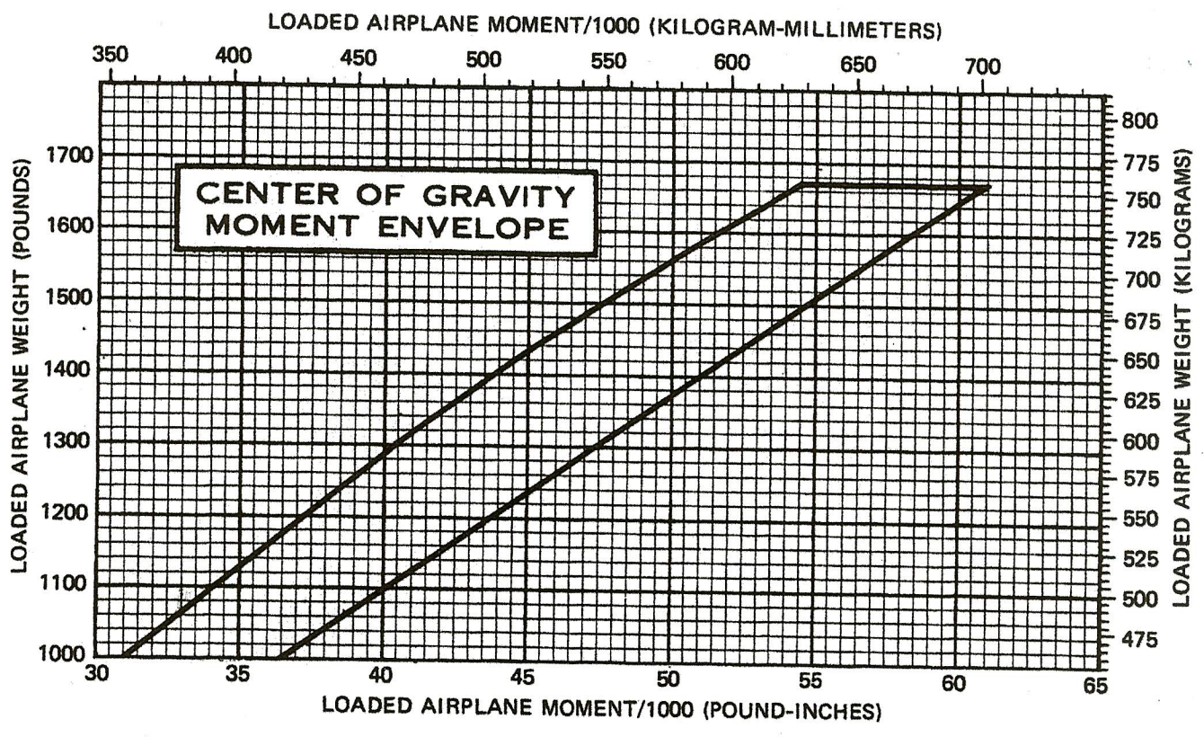
Figure 6-8. Center of Gravity Moment Envelope
